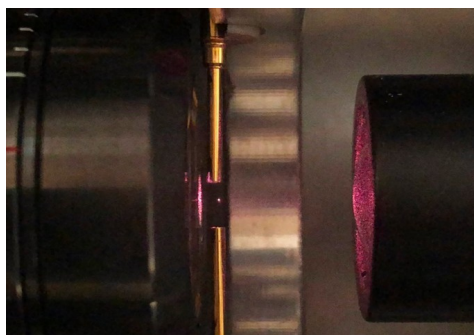
(left) Artist view of the levitation of two coupled particles (src: npg group). (right) A 70 nm nanoparticle trapped in vacuum (bright red spot) by a highly focused laser through an objective (on the left).
