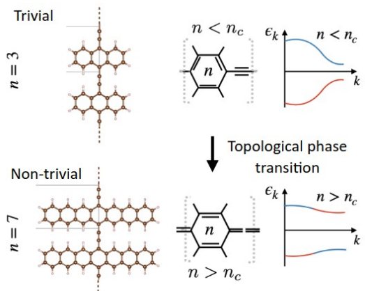
Fig. 3 : Topological phase transition of polyacene polymers [19]
