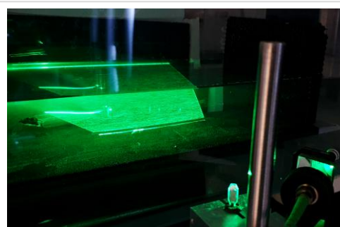
Preliminary experimental set-up at LIPhy. Fish visible in the light sheet.
