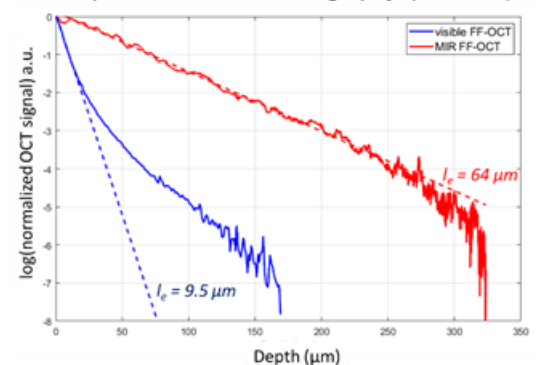
Figure 2: FF-OCT measurement of the extinction mean-free-path l_e of white acrylic paint in the MIR spectral range (MWIR, 3-5 \mu\text{m} ) compared to the same measurement at visible wavelengths.
