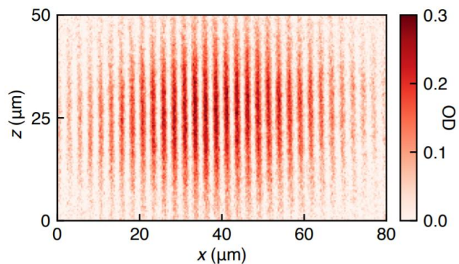
Figure 1: array of individual 1D tubes. The distance between two neighboring tubes is 2.5\mu\text{m} and each tube contains typically a hundred atoms. Figure from de Danilo et al. , PRL 127, 113602 (2021) .
